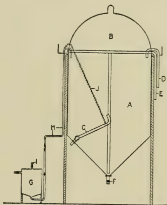
FIG. 114.—Apparatus for the Acid-Purification of Petroleum Distillates.
